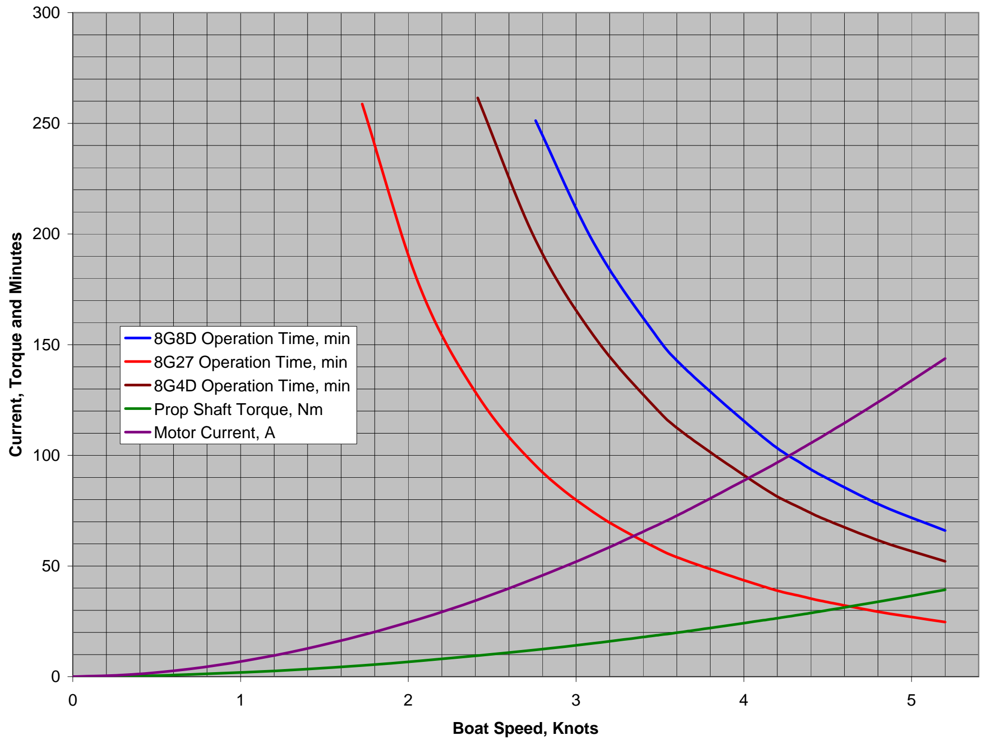
Load Current vs Boat Speed (Bristol 27'). Prop 3 Blade, 12" Dia, 7" Pitch. MK Battery Bank
